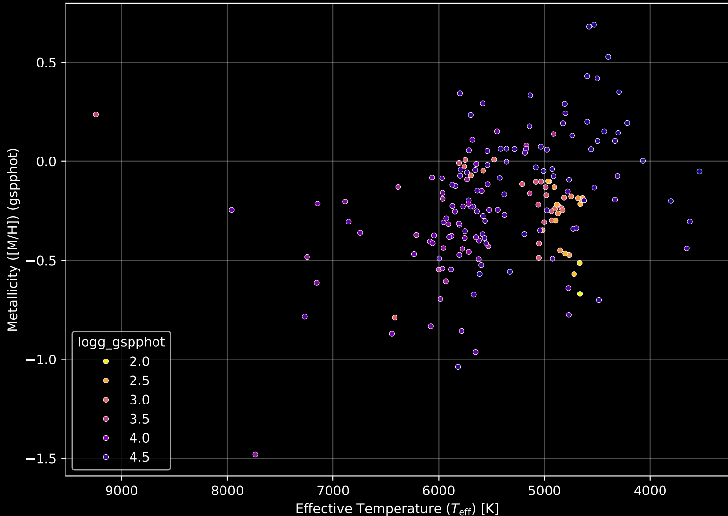
APOGEE DR17 Field: [196+40_MGA] Stellar Population Parameters (n= 185)
