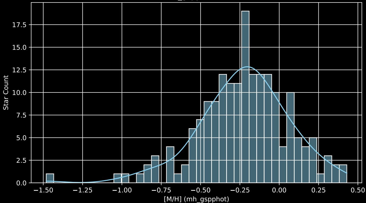
APOGEE DR17 Field: [196+40_MGA [M/H] (mh_gspphot) (n= 182)
