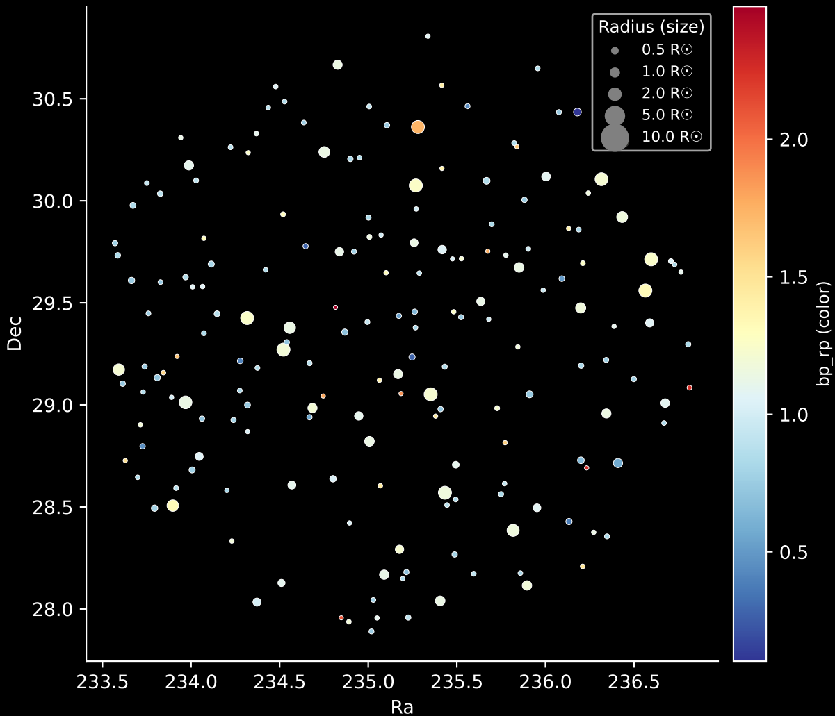
APOGEE DR17 Field: [196+40_MGA] Stars: 185
