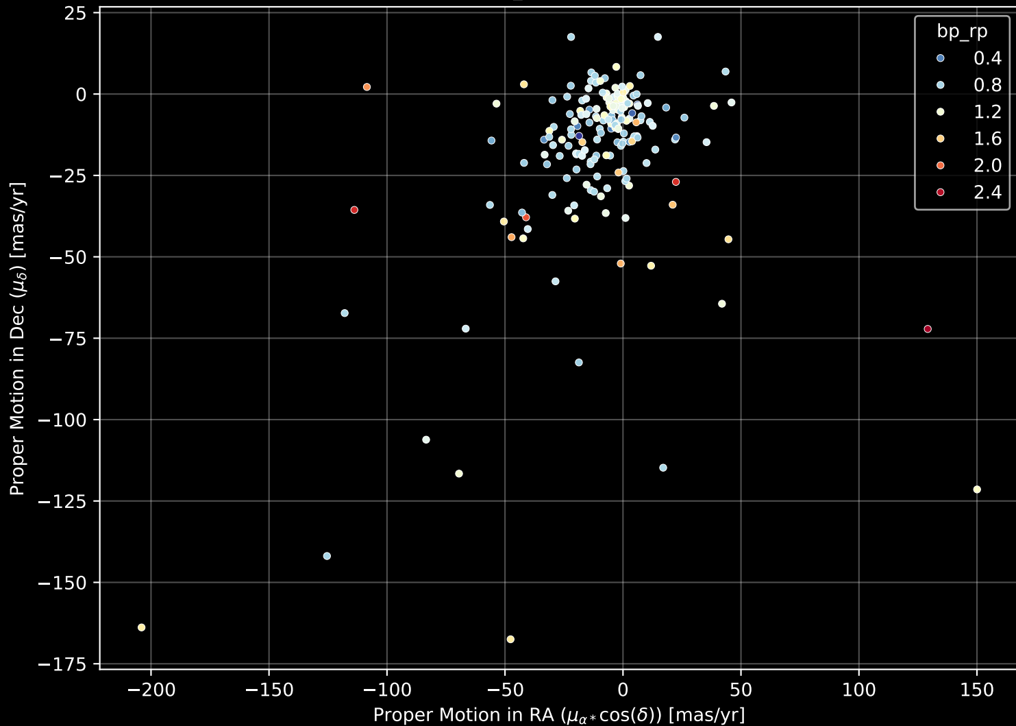
APOGEE DR17 Field: [196+40_MGA] Proper Motion Diagram (n= 185)
