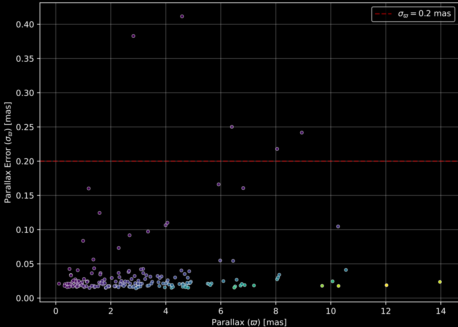
APOGEE DR17 Field: [196+40_MGA] Parallax Quality (n= 185)
